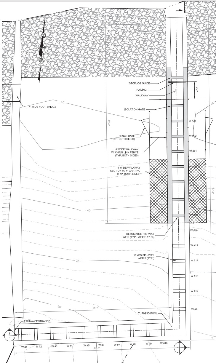
FISHWAY PLAN VIEW SCALE: 1/4" = 1'-0"
