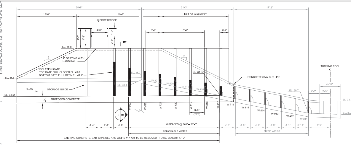
4 FISHWAY CENTERLINE PROFILE - WEIRS #11 - #23 SCALE: 1/4" = 1'-0"
