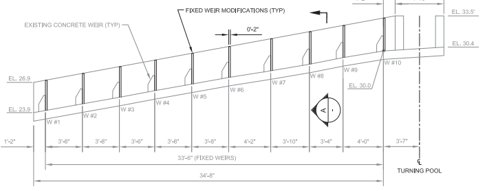
3 FISHWAY CENTERLINE PROFILE - WEIRS #1 - #10 SCALE: 1/4" = 1'-0"
