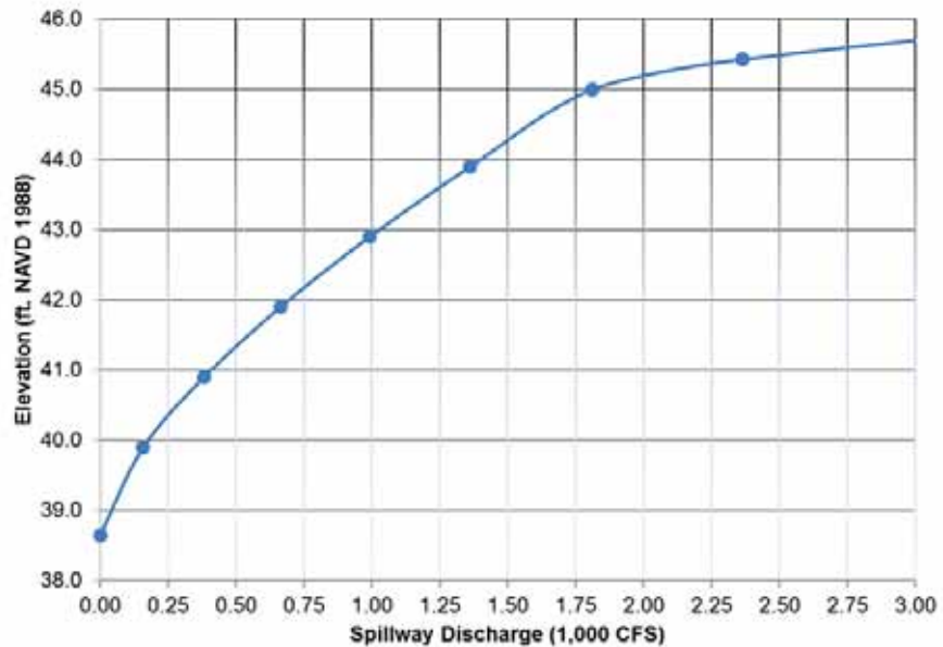
Figure 4-3 Reservoir Dam Spillway Crest Gate Discharge Rating Curve
