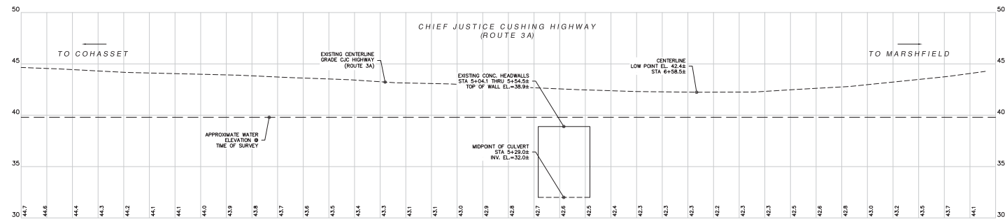
PROFILE C.J.C. HIGHWAY (ROUTE 3A)
