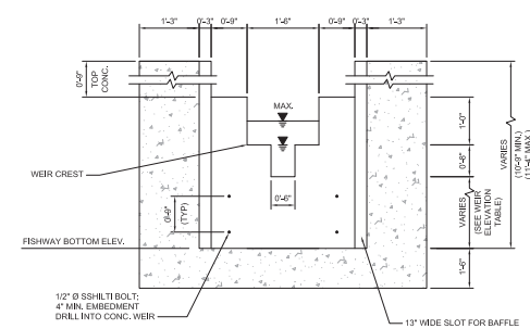
B TYPICAL REMOVABLE WEIR SCALE: NTS
