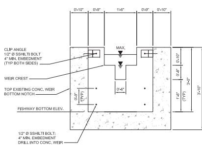
A TYPICAL FIXED WEIR MODIFICATION SCALE: 3/4" = 1'-0"
