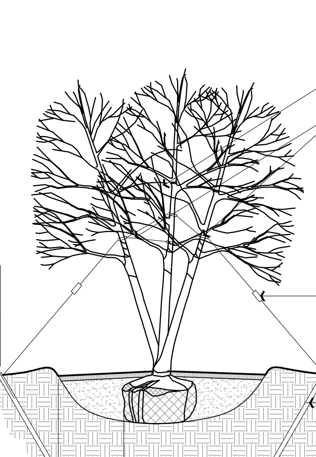
SHRUB DETAIL 1/2" = 1'-0" 3229335.00.02
