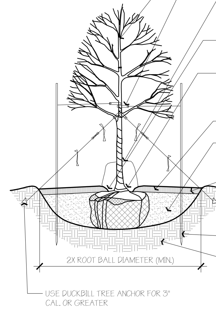
SHADE / FLOWERING TREE DETAIL 1/2" = 1'-0" 3229345.01.01
